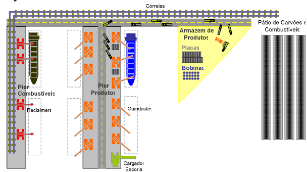
Figure 2: Harbor Layout
